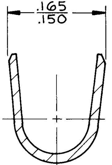
SECTION B-B
